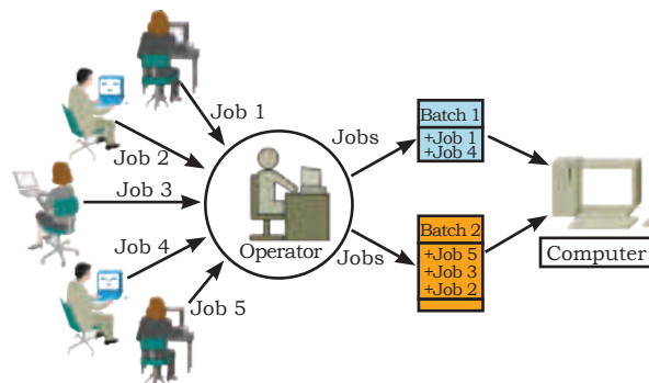
Fig. 4.20: Batch processing
