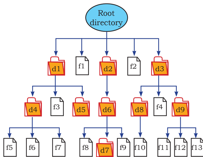
Fig. 4.7: File management
