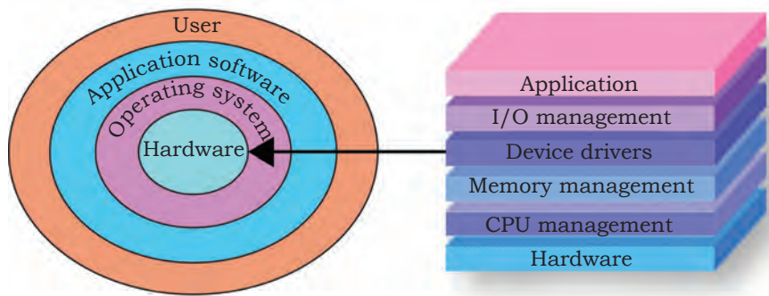
Fig. 4.1: Resource management
