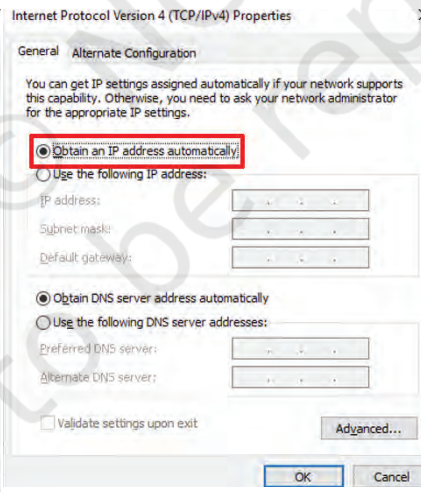
Fig. 5.28: IPv4 properties
