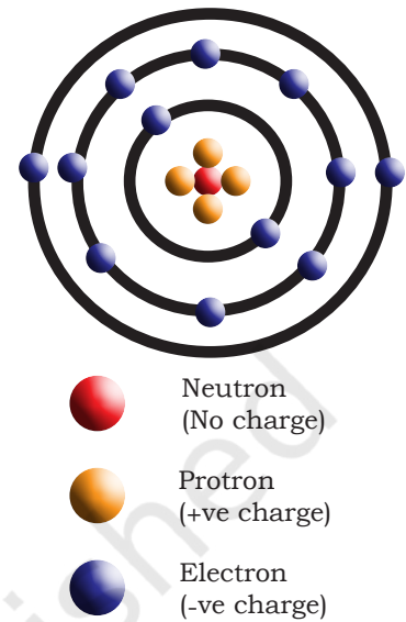
Fig. 1.1: Atomic structure
