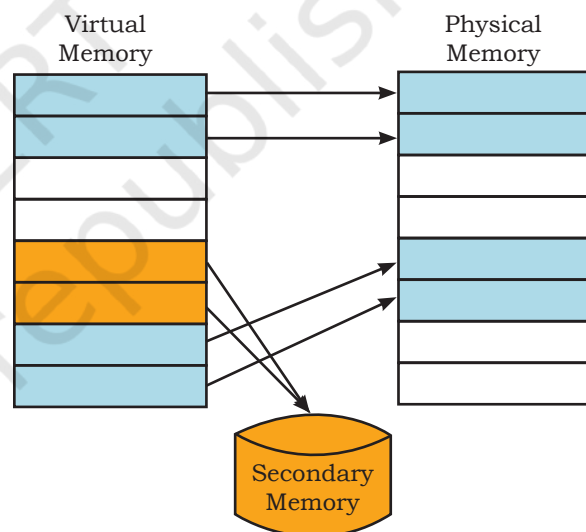
Fig. 4.10: Virtual storage
