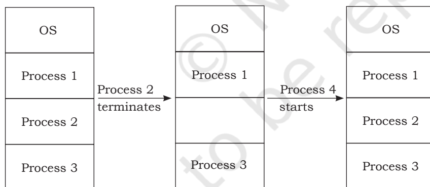
Fig. 4.4: Memory management
