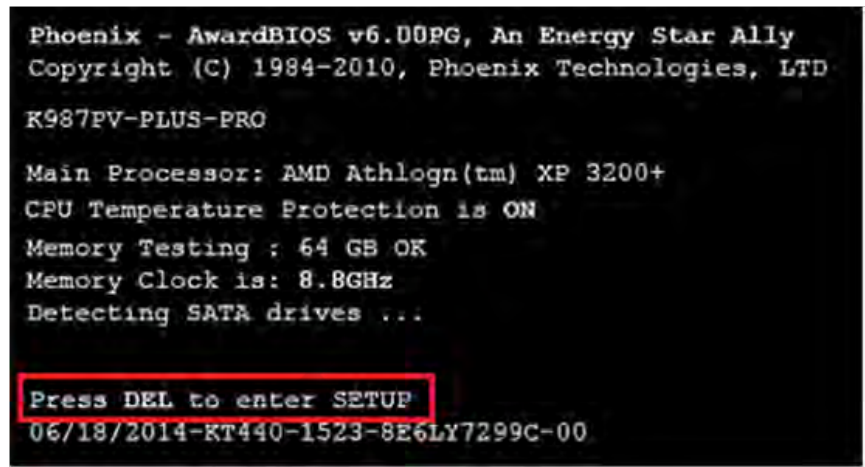
Fig. 7.24: Entering setup
