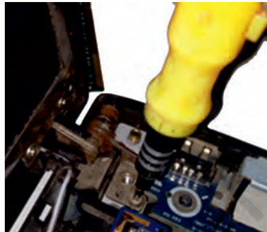
Fig. 12.69: Remove screws fastening display hinge
