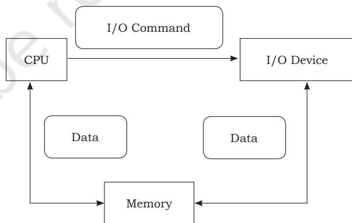
Fig. 4.6: Device management
