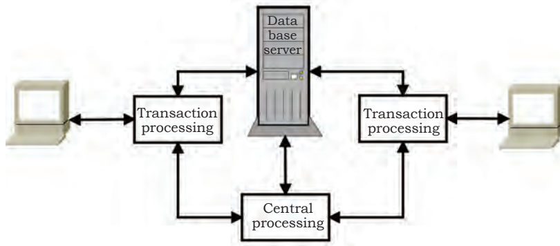
Fig. 4.21: Online processing
