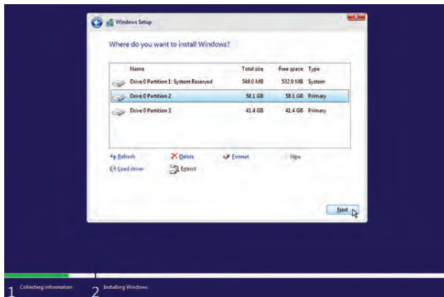
Fig. 5.10: Partition window
