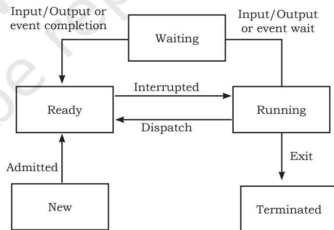
Fig. 4.2: Input/Output management
