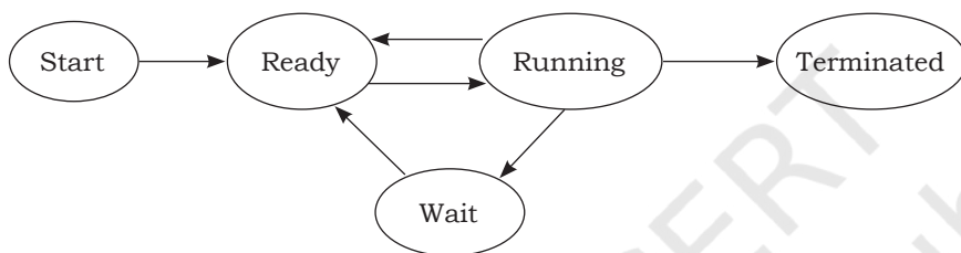
Fig. 4.5: Process management
