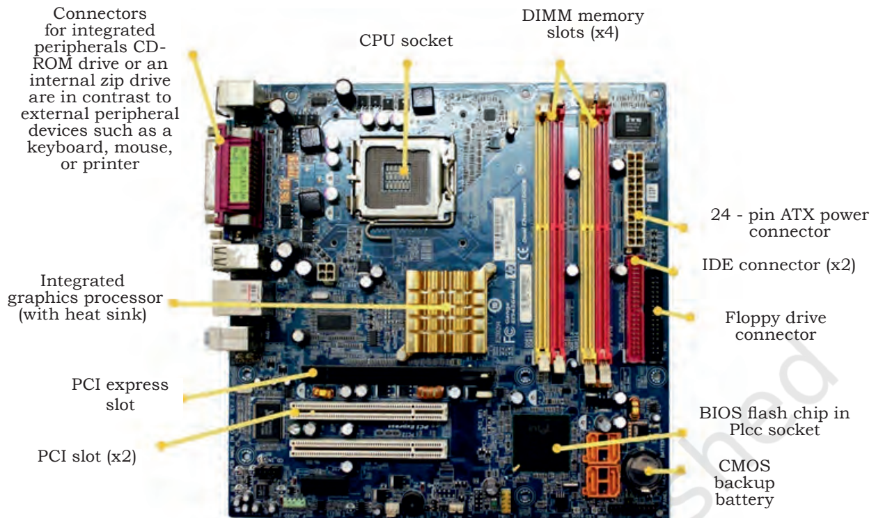
Fig. 7.1: Internal structure of motherboard
