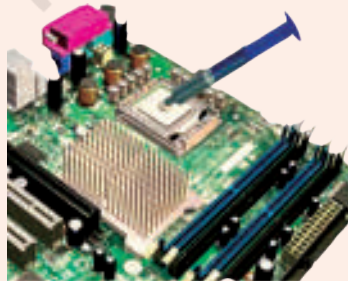
Fig. 2: Applying thermal compound on CPU
