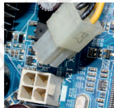
Fig. 12.19: Plug-in 4-pin AUX power connector to motherboard
