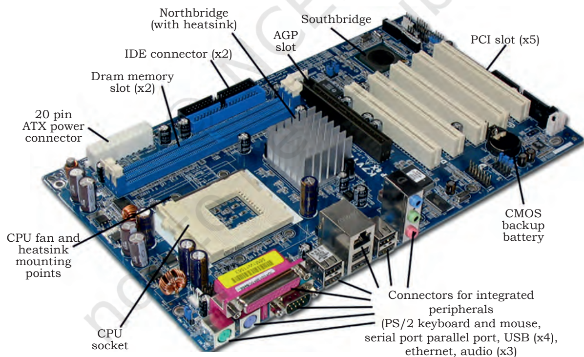
Fig. 7.3: Motherboard components
