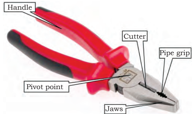
Fig.11.6: Combination pliers
