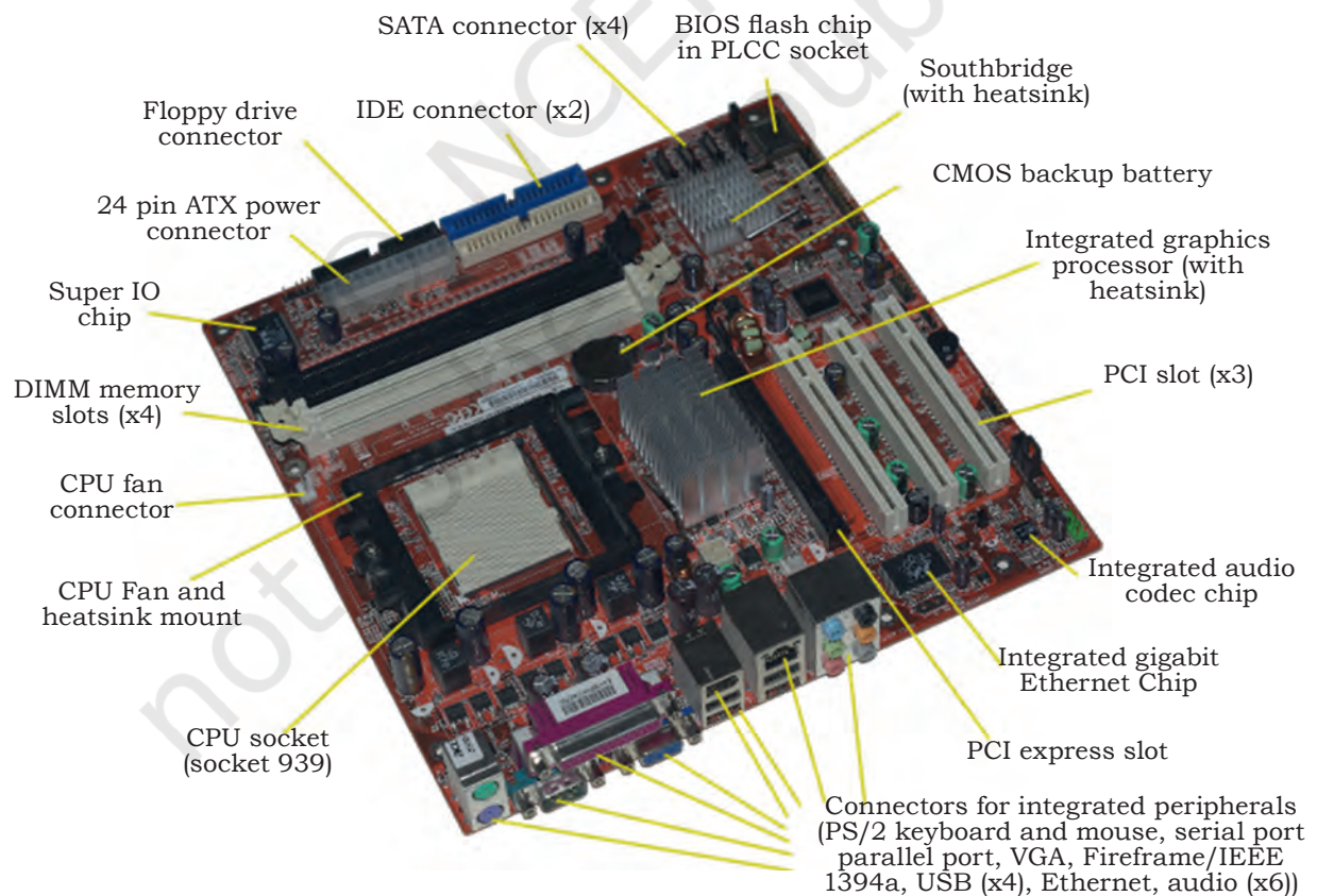
Fig. 7.2: Integrated motherboard
