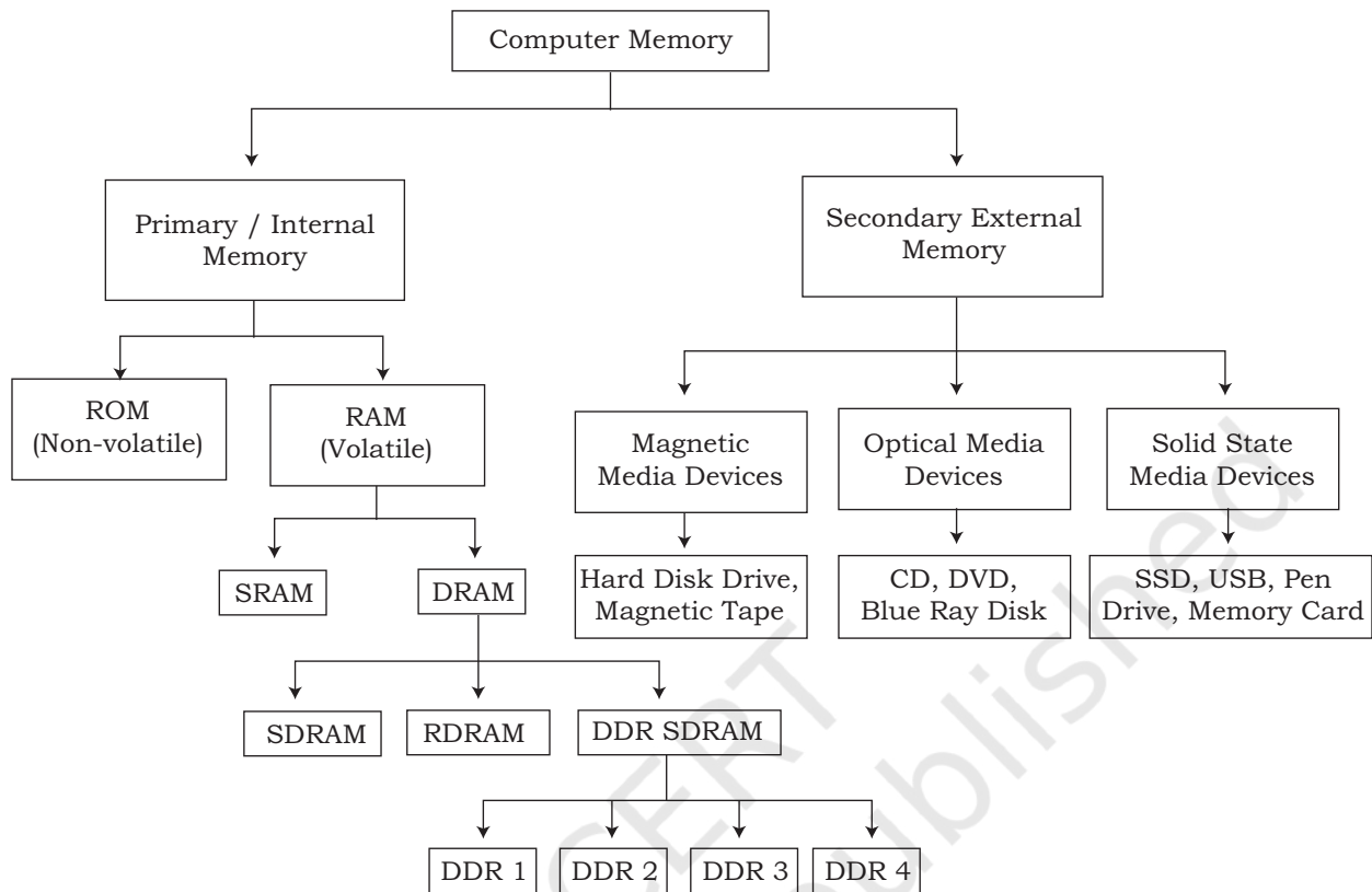
Fig. 9.1: Different types of memory
