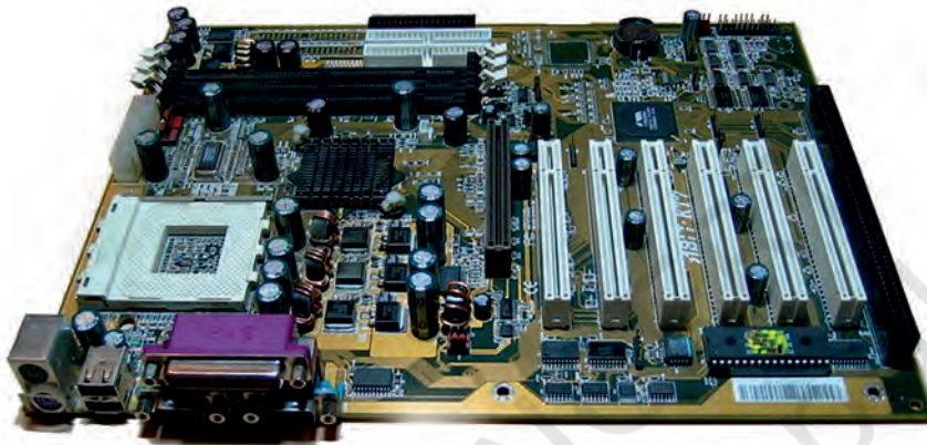
Fig. 7.7: LPX form factor
