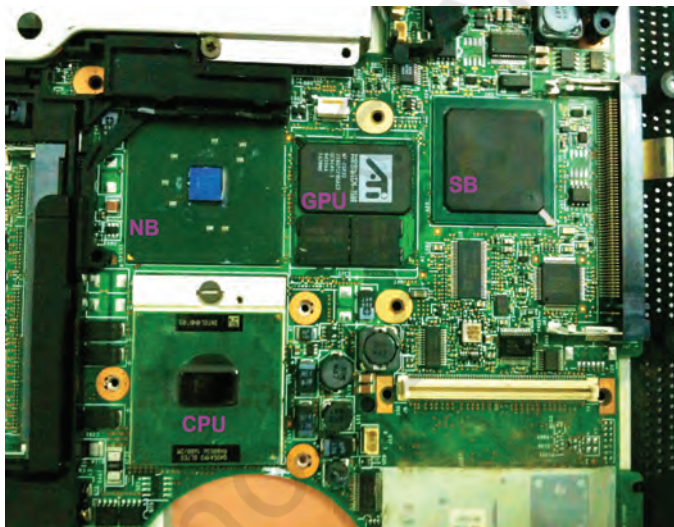
Fig. 7.10: Chipset north and southbridge
