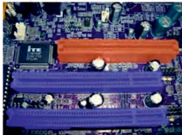
Fig. 7.12: AGP slots
