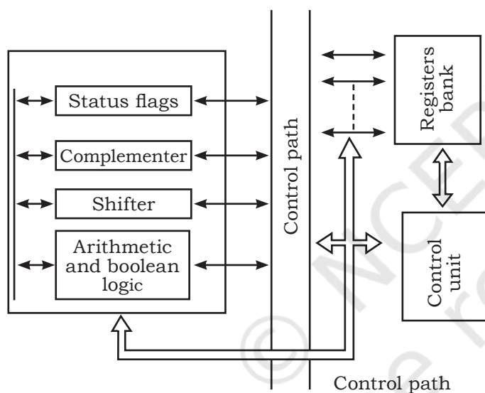
Fig. 8.8: Internal organisation of CPU
