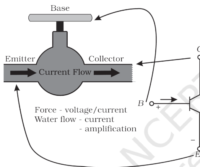
Fig. 1.12: Analogy showing a tap as the base of the transistor
