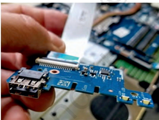
Fig. 12.66: Remove USB LED status board
