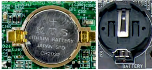
Fig. 7.11: Lithium battery and its socket
