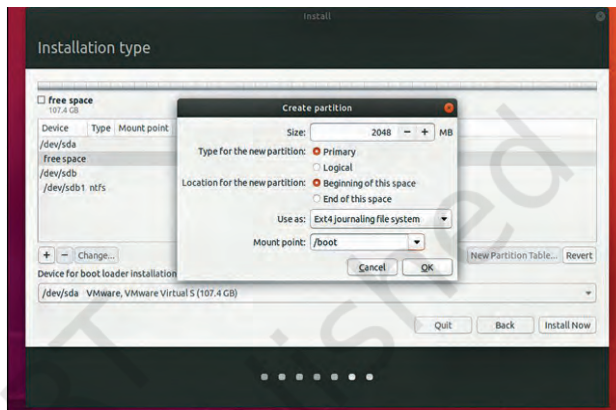
Fig. 6.9: Creating '/' boot partition
