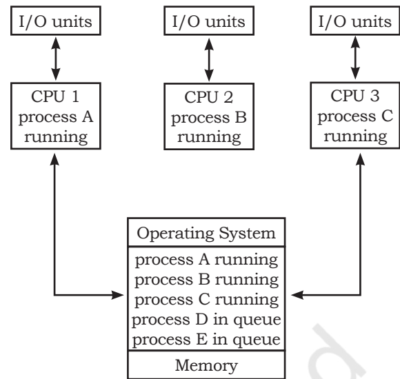
Fig. 4.18: Multiprocessing OS
