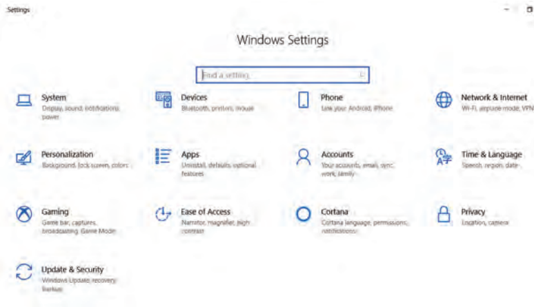
Fig. 5.14: Window setting
