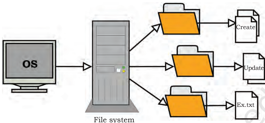
Fig. 4.3: Data management
