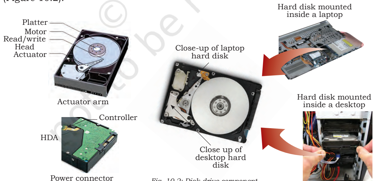
Fig. 10.2: Disk drive component
