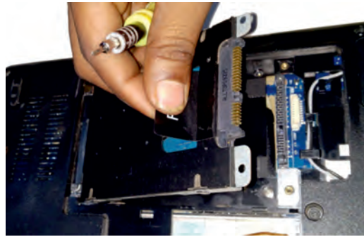
Fig. 12.64: Disconnect SATA cable
