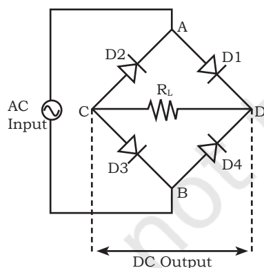
Fig. 1.26: Construction of bridge rectifier circuit
