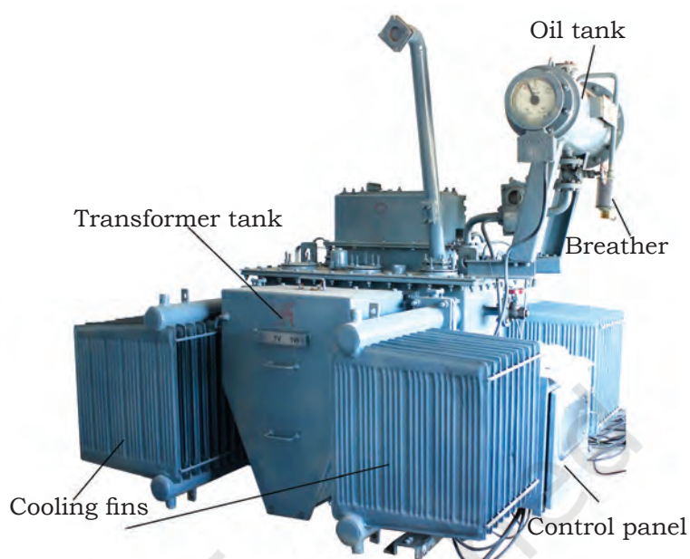
Fig. 1.21: Transformer parts
