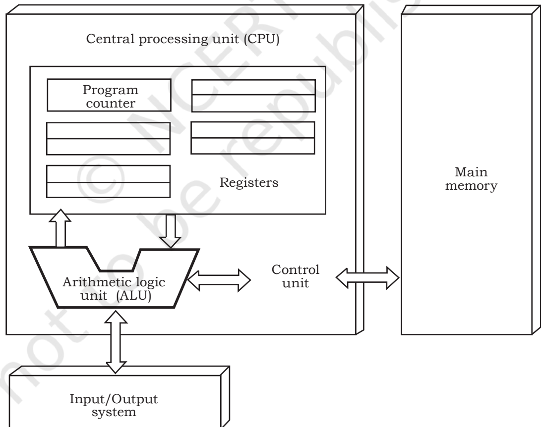
Fig. 8.7: Organisation of register
