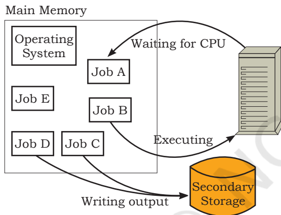
Fig. 4.16: Multi-programming with three programs
