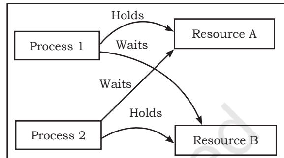
Fig. 4.9: Deadlock prevention
