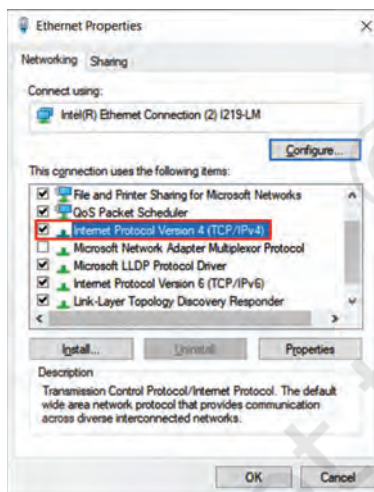
Fig. 5.27: Selecting IPv4
