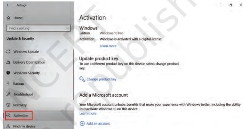
Fig. 5.16: Selecting activation
