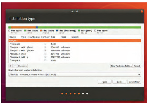
Fig. 6.12: Begin installation
