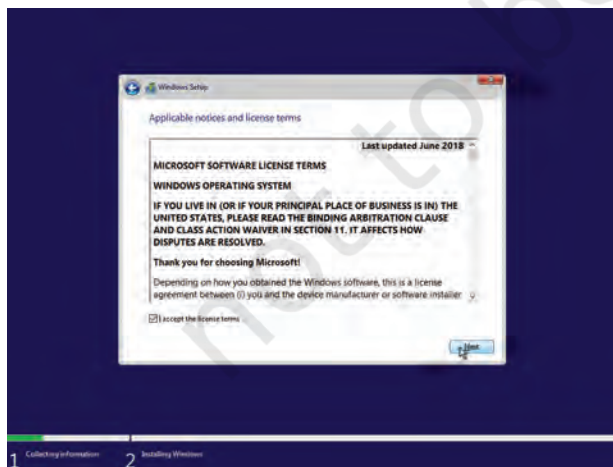
Fig. 5.8: License terms
