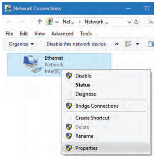
Fig. 5.26: Ethernet properties
