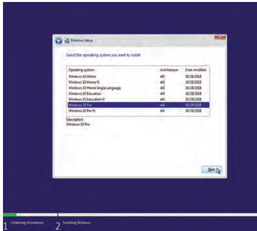
Fig. 5.6: Collecting information
