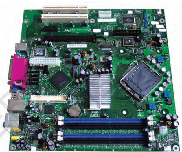
Fig. 7.8: BTX form factor
